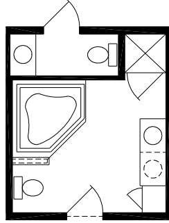
Master Bath Option WVB2 Roman Tub and Shower (Pull Down Stairs Relocated to Master Bedroom Closet)
