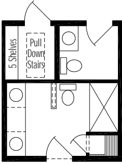
Master Bath Option WVB1 5' Shower
