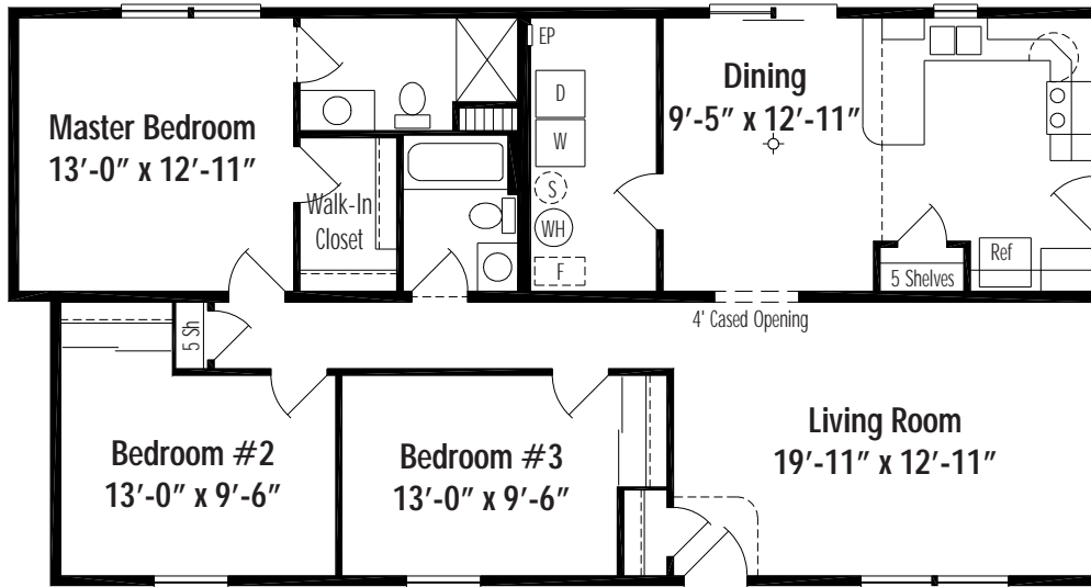
Glenmont C Crawl Space 27'-4" x 50/52', 1394 Sq. Ft. Living Area
