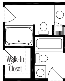
Master Bath Option CVB2 Garden Tub
