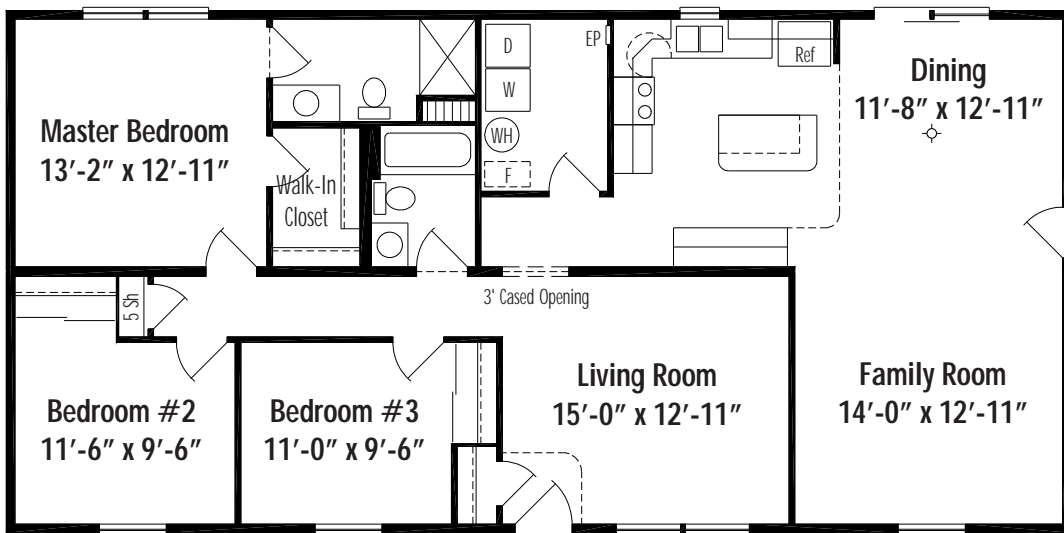
Cedarville A Crawl Space 27'-4" x 56', 1531 Sq. Ft. Living Area
