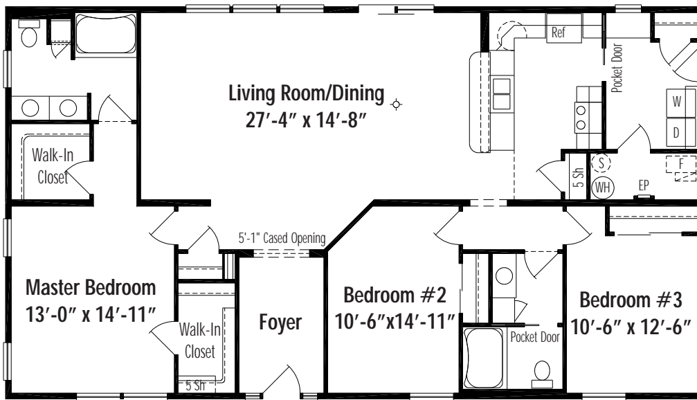
Carmel A Crawl Space 31'-4" x 56' • 1754 Sq. Ft. Living Area
