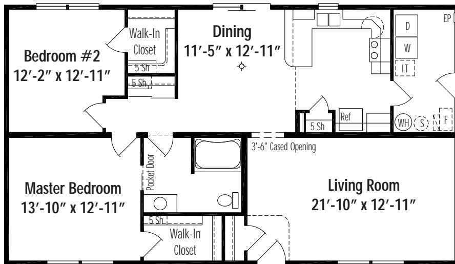
Bexley A Crawl Space 27'-4" x 48', 1312 Sq. Ft. Living Area
