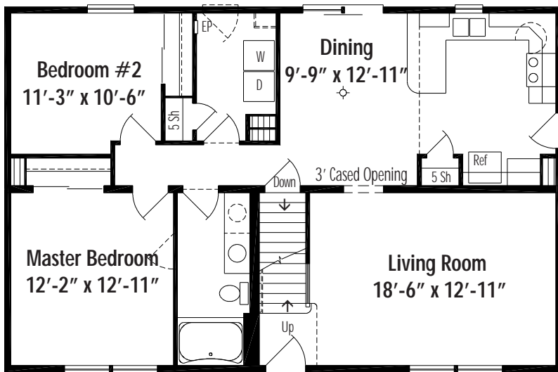
Walden B Basement 27'-4" x 42', First Floor Living Area 1148 Sq. Ft.
