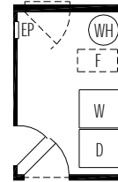
Utility Option WLU1 Alternate Utility Arrangement (Crawl Space Plan Only)
